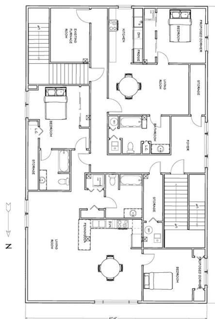
Proposed 2 nd Floor Plan
