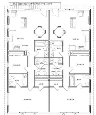
Proposed 2 nd Floor Plan
